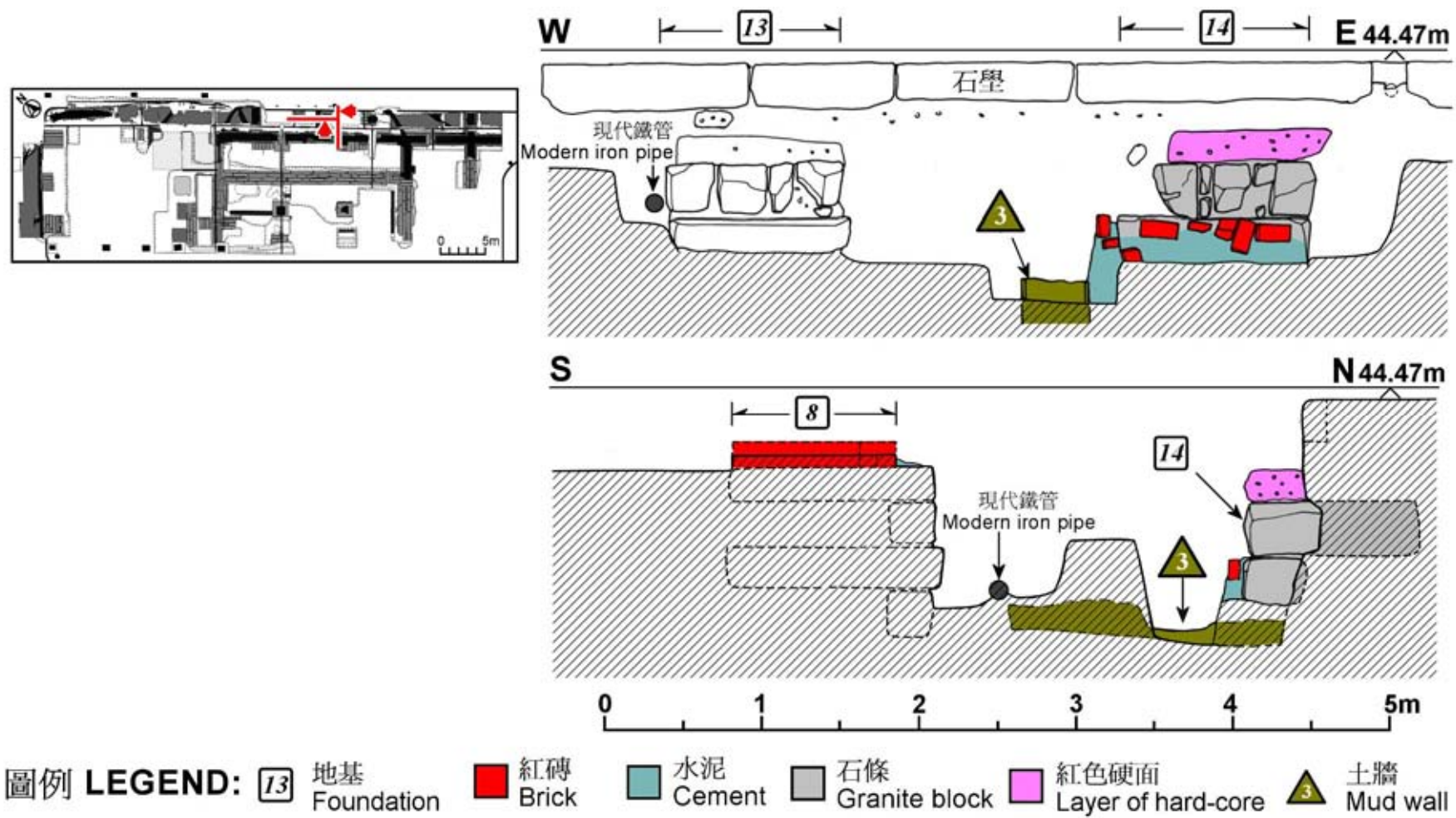
Fig 29 Side Views of Foundation (14)
