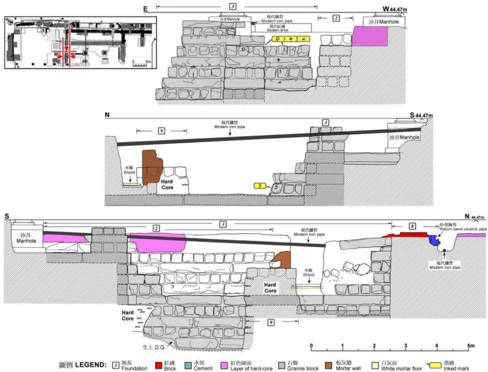
Fig 18 Side Views of Foundation (3)
