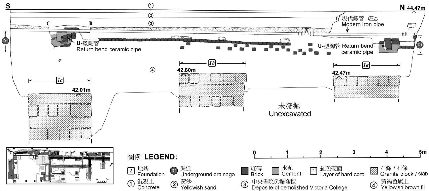
Fig 12 Plan and Sections of T4
