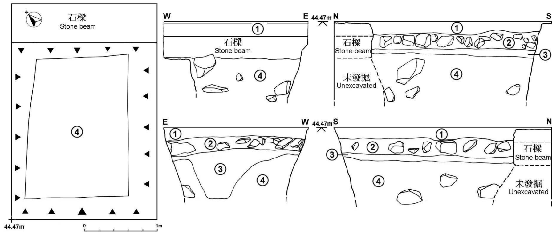
Fig 10 Plan and Sections of T8
