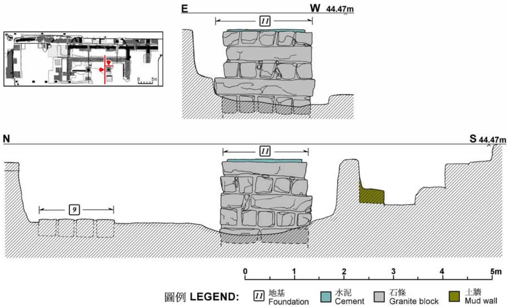
Fig 26 Side Views of Foundation (11)
