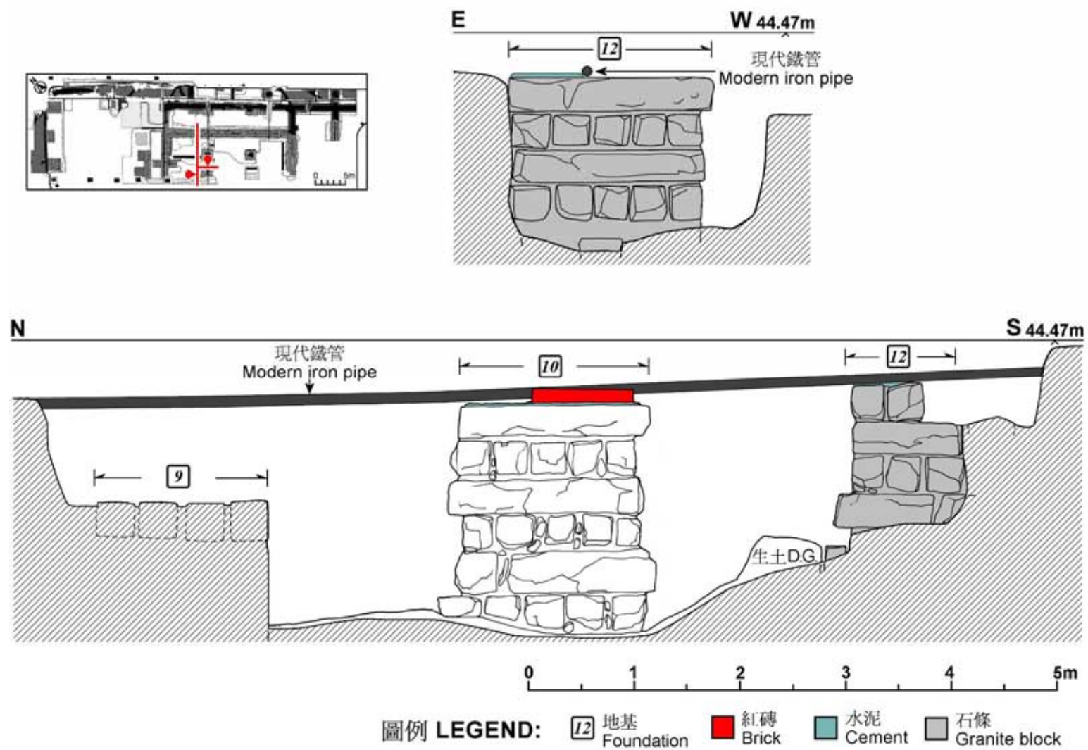
Fig 27 Side Views of Foundation (12)
