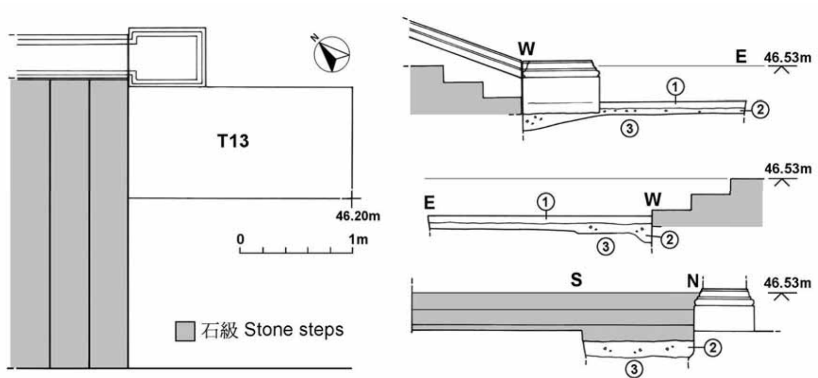
Fig 8 Plan and Sections of T13
