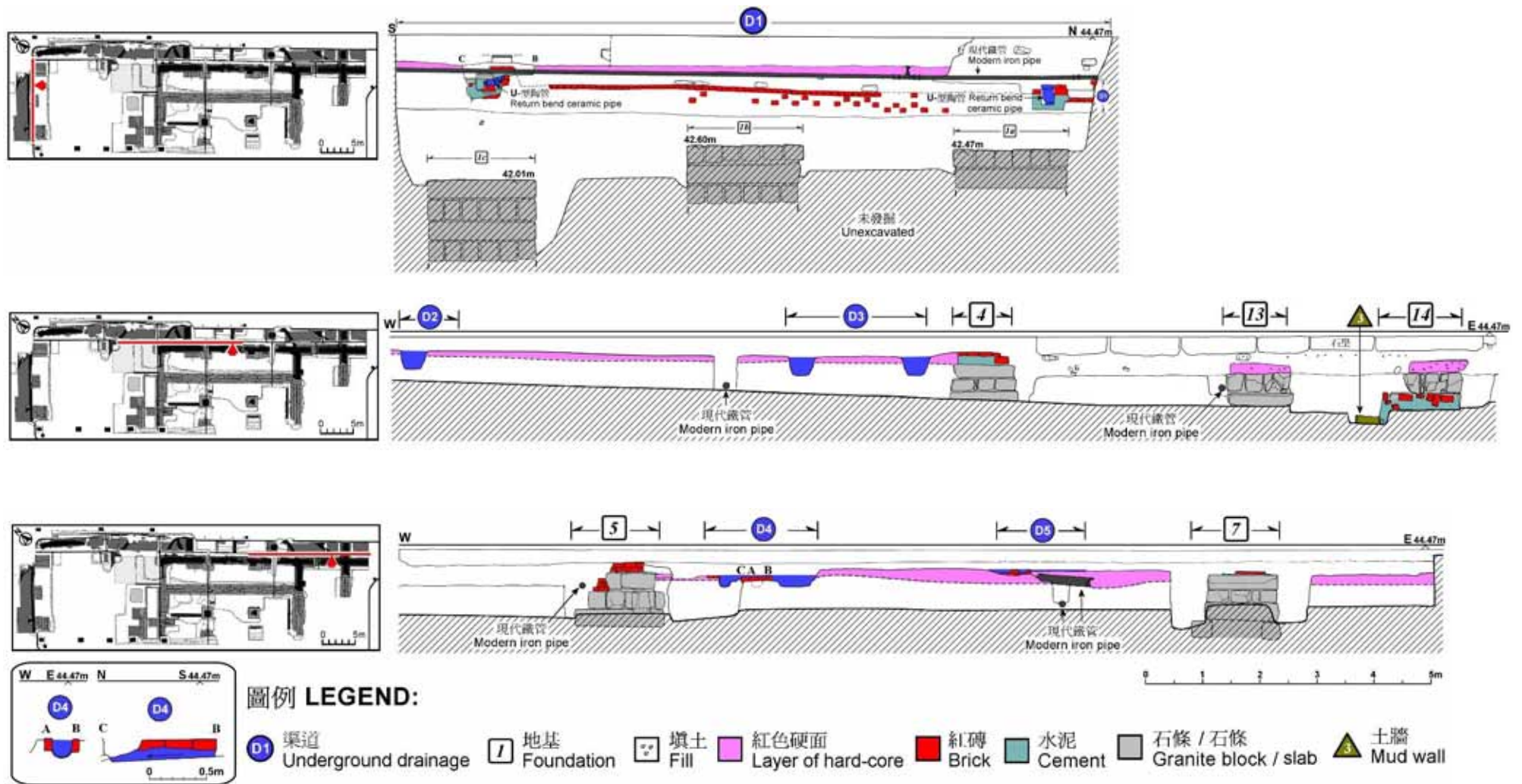
Fig 15 Sections of the Underground Drainage (D1-D5)
