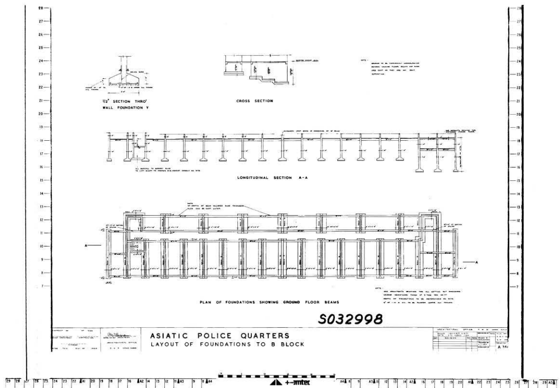
27. Layout of Foundations to Block B of Asiatic Police Quarters, 1950
