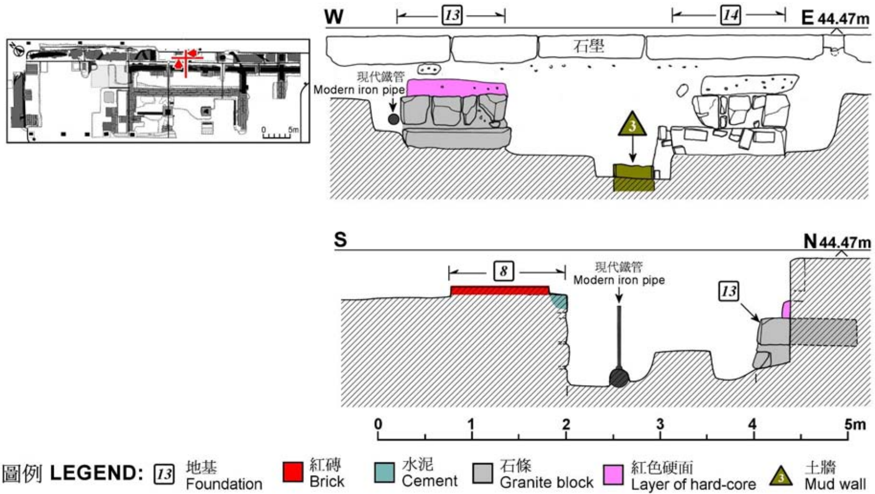
Fig 28 Side Views of Foundation (13)
