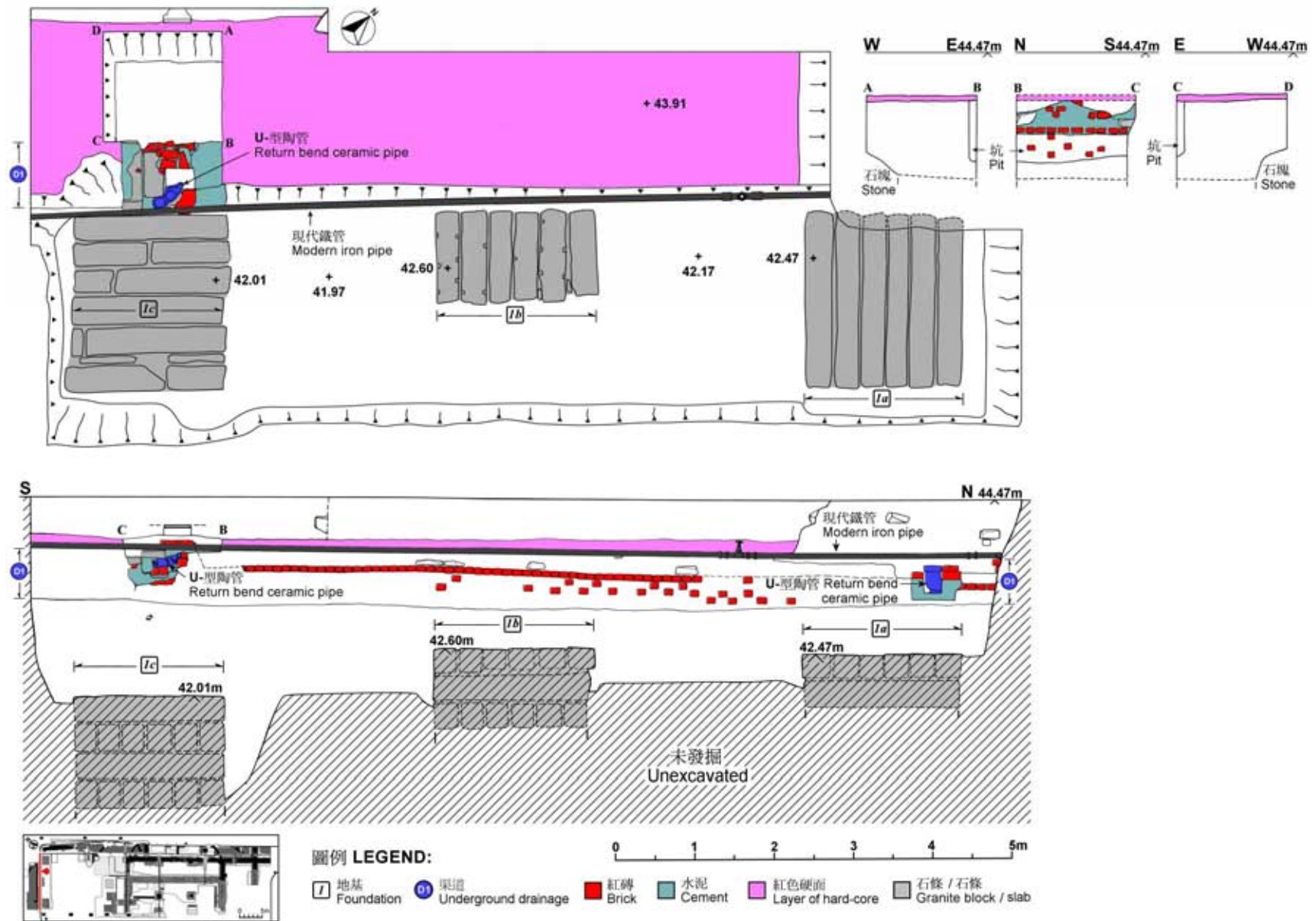
Fig 16 Plan and Side View of Foundation (1)
