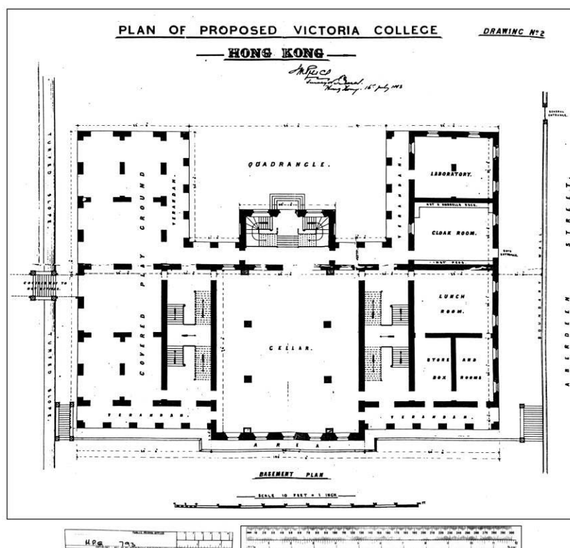
16. Basement Floor Plan of Victoria College, 1883
