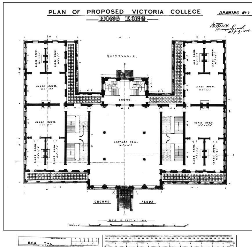
17. Ground Floor Plan of Victoria College, 1883
