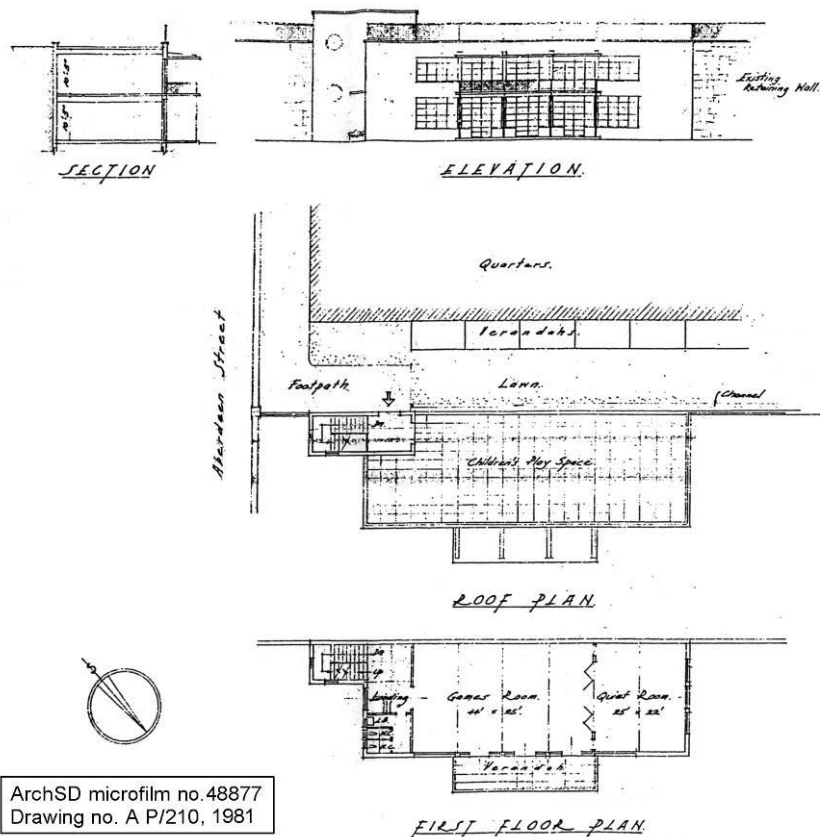
30. Elevation and Floor Plan of Central Junior Police Call Clubhouse, 1981
