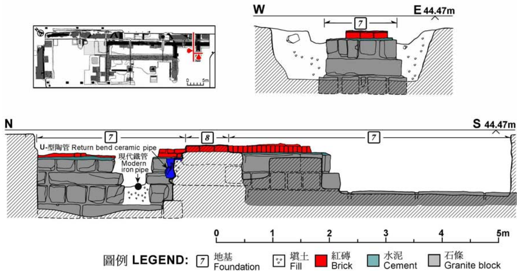
Fig 22 Side Views of Foundation (7)
