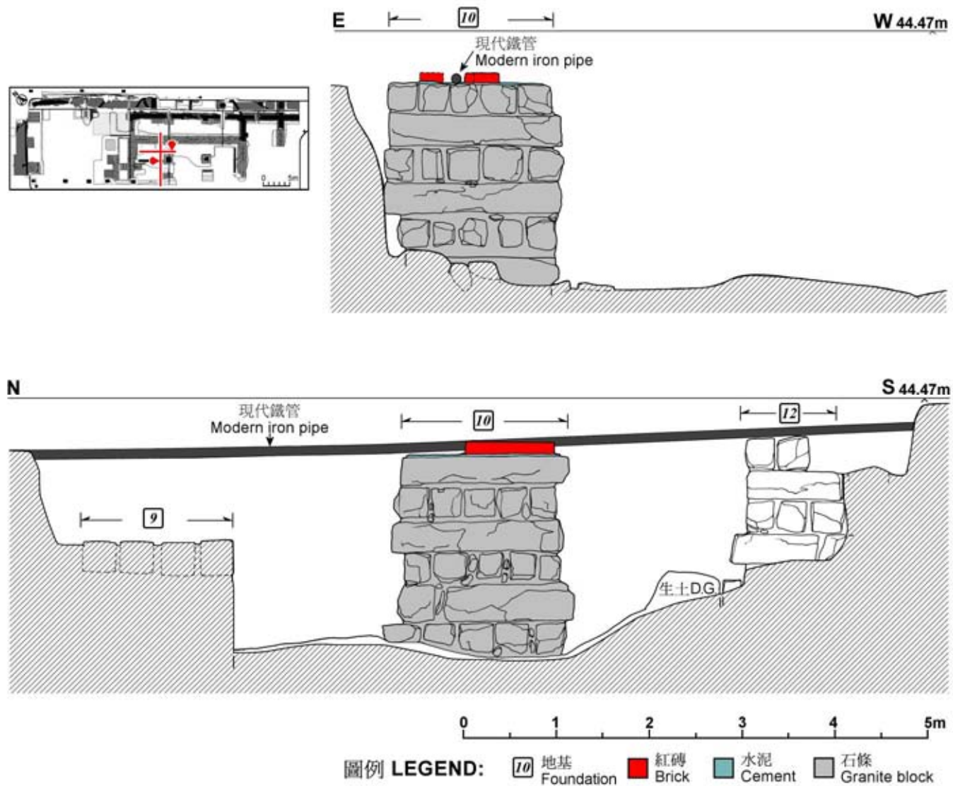
Fig 25 Side Views of Foundation (10)
