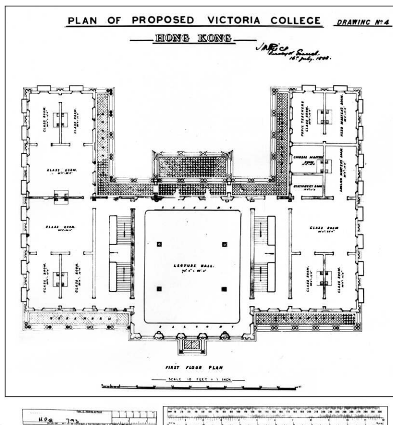
18. First Floor Plan of Victoria College, 1883
