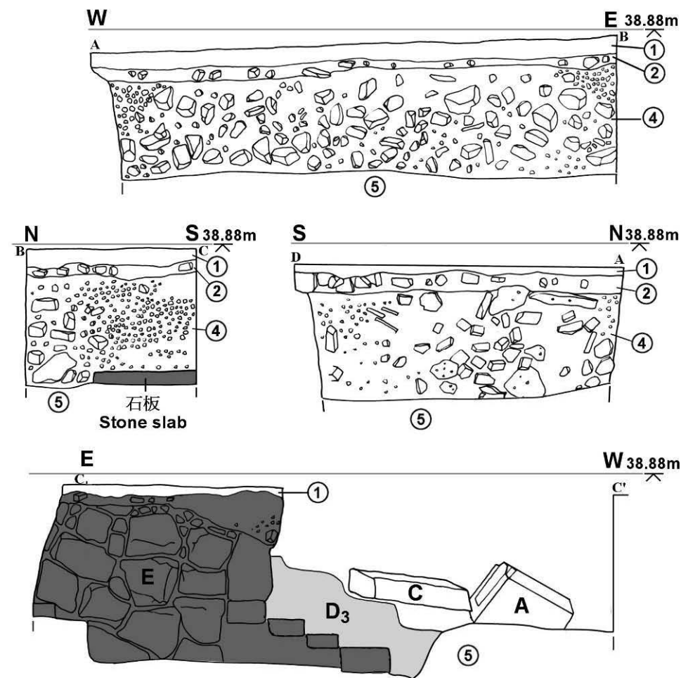
Fig 6 Plan and Sections of T5
