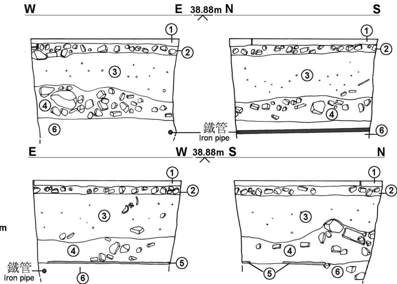
Fig 7 Plan and Sections of T15
