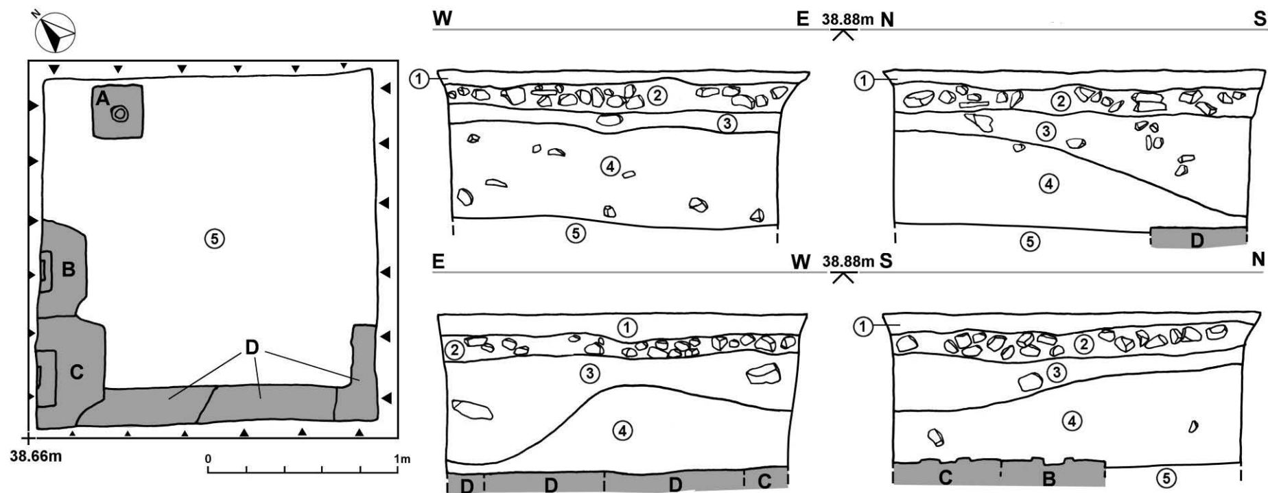
Fig 4 Plan and Sections of T1
