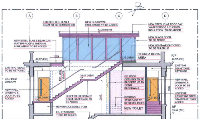
SECTION C-C 1:100
